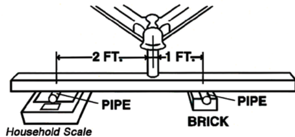
Method for Measuring Trailer Tongue Weight (TW) Multiply the reading on the scale by 3.
