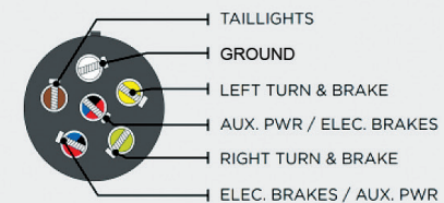
6 ROUND
