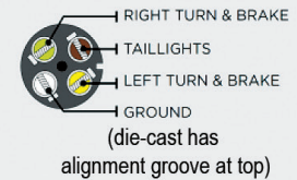
4 ROUND (small)
