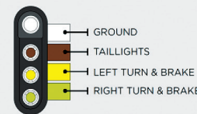
4 FLAT
