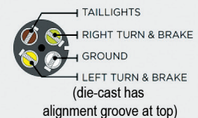
4 ROUND (small)
