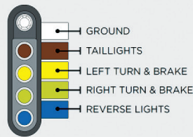
5 FLAT
