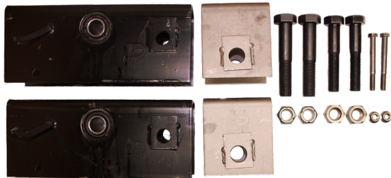
TAP8181 HAP-203-01 Tandem axle w/ 3" wide springs, 38" spacing $371.95
