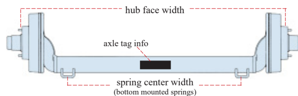
Drop Axle
