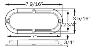
Flange mount
