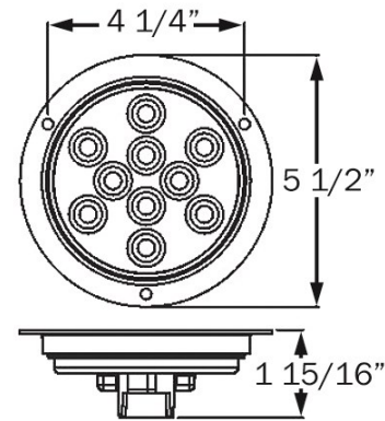
Flange mount
