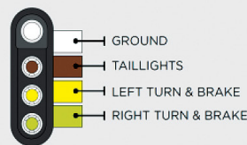
4 FLAT
