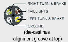
4 ROUND (small)
