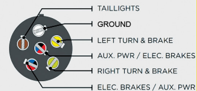
6 ROUND
