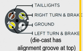
4 ROUND (small)
