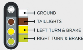
4 FLAT
